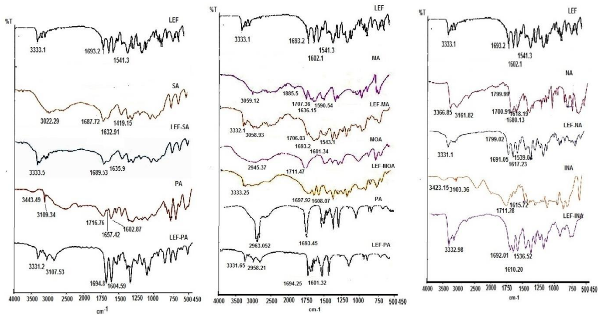
Figure S4. FT-IR spectra of LEF, coformers and eutectics of LEF
