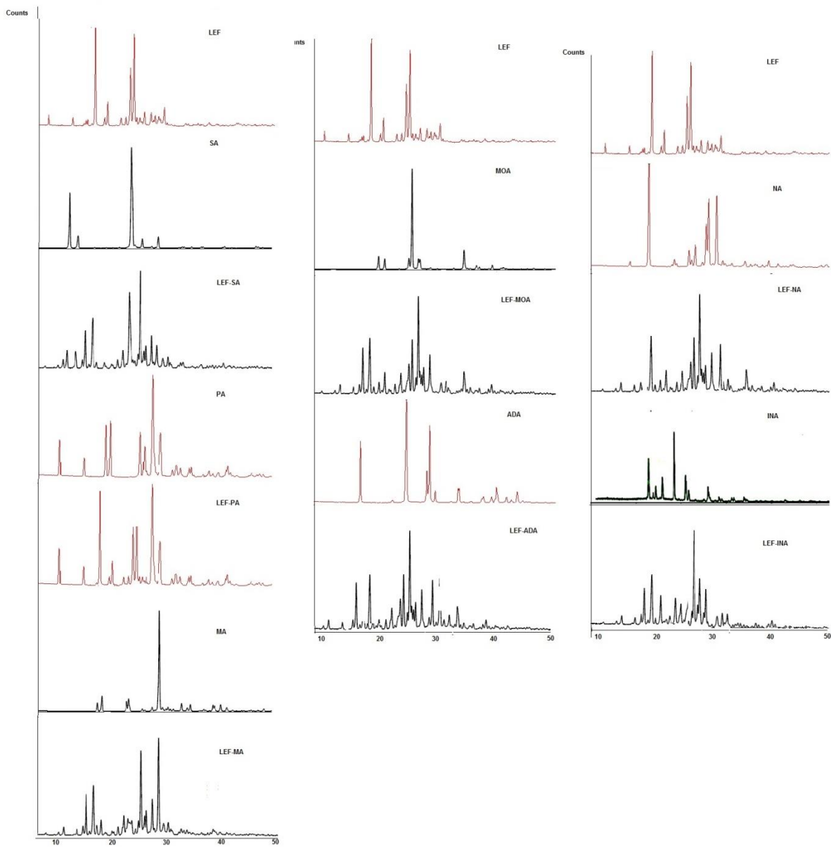
Figure S5. PXRD pattern of LEF, coformers and eutectics of LEF
