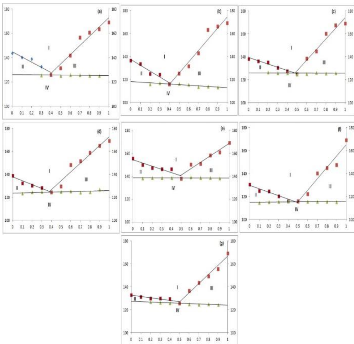
Figure S3. Phase diagrams of eutectics of (a) LEF-MA (b) LEF-SA (c) LEF-PA (d) LEF-MOA (e) LEF-ADA (f) LEF-NA (g) LEF-INA, where x axis represent mole fraction of LEF and y axis represents temperature in °C.
