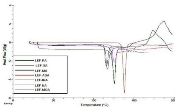
Figure S2. Overlay of DSC thermograms of eutectics of LEF.
