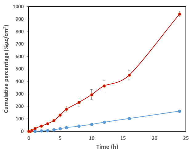
Figure 3. Transdermal permeation profiles of TZN solution and the optimized TNCUBs-gel across rat skin over 24 h
