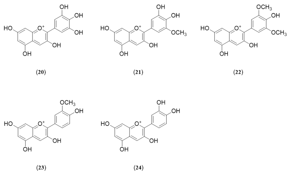
Figure 3. Anthocyanins isolated from V. Arctostaphylos
