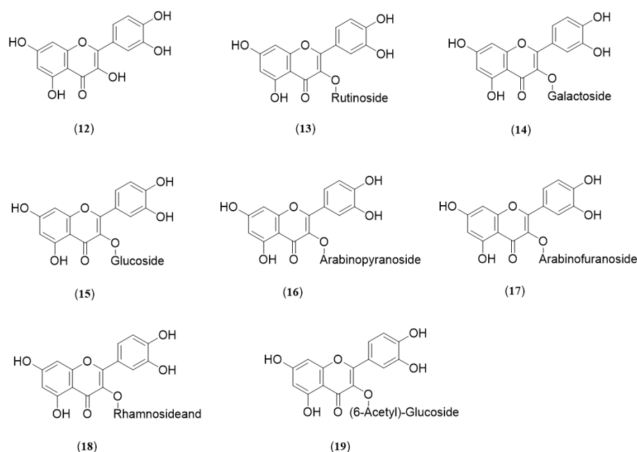
Figure 2. Flavonoids and their glycosides isolated from V. Arctostaphylos
