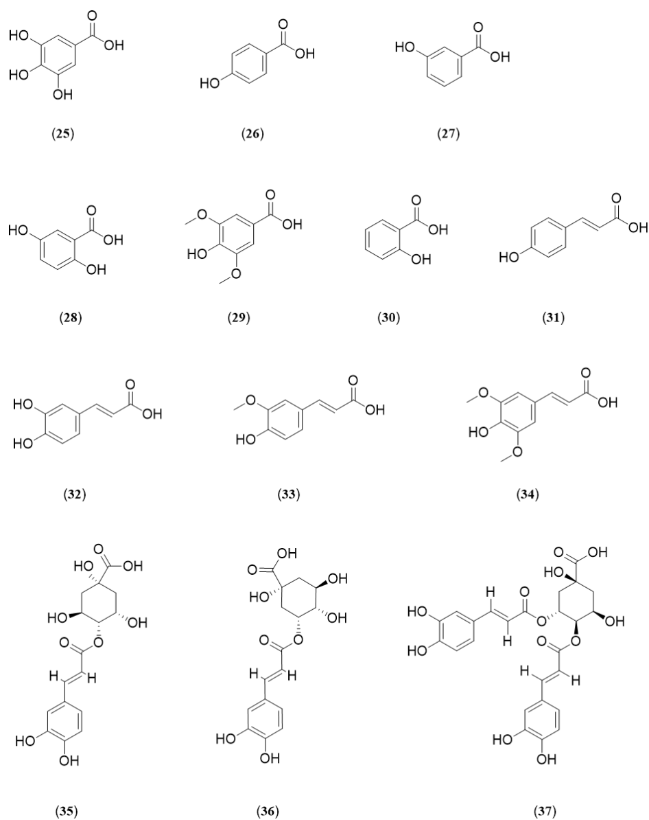
Figure 4. Phenolic acids isolated from V. arctostaphylos
