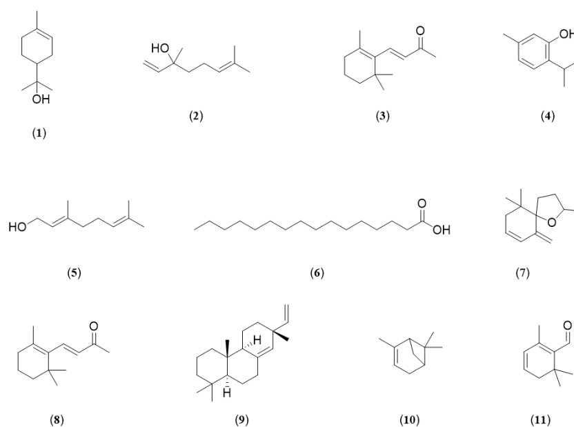
Figure 1. Volatile compounds isolated from V. Arctostaphylos
