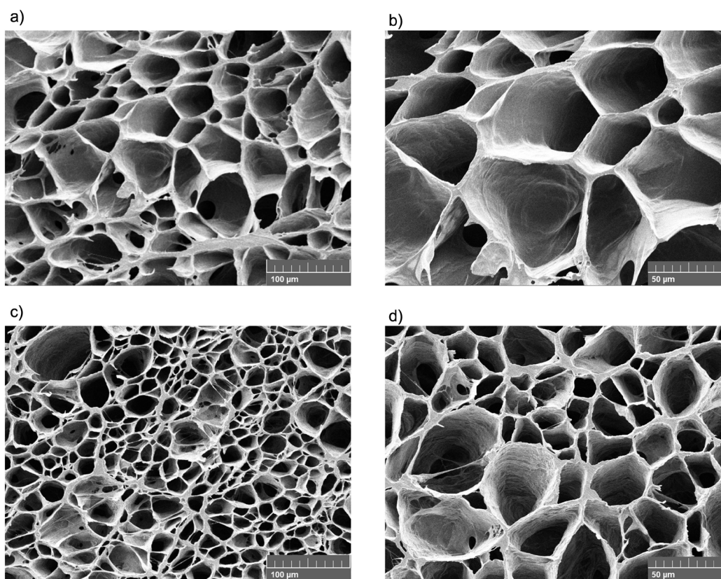
Figure 6. SEM images of (a-b) PVA-CMC hydrogel and (c-d) Res/GA-IC loaded PVA-CMC hydrogel in the swollen state at 500× and 1k× magnification
