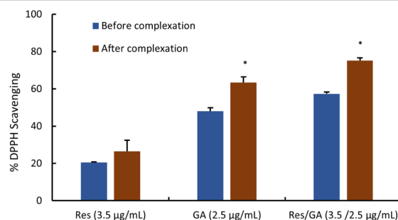
Figure 5. DPPH scavenging activity of RES, GA, and their synergistic combination before and after inclusion complex formation with HP- \beta -CD (*Significant difference compared to prior to complexation, P < 0.05 )
