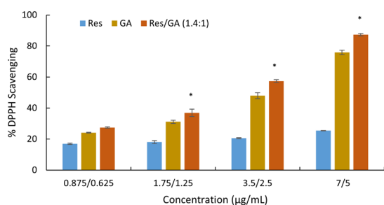
Figure 3. Synergistic antioxidant activity of Res/GA at a weight ratio of 1.4:1 compared to individual Res and GA. (* Significant difference compared to single Res and GA, P < 0.05 )
