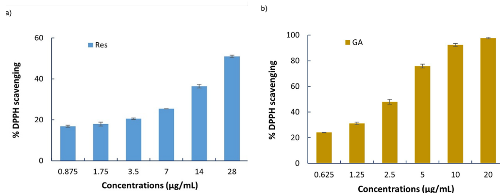
Figure 1. Percentage of DPPH scavenging activity of (a) Res; (b) GA at different concentrations
