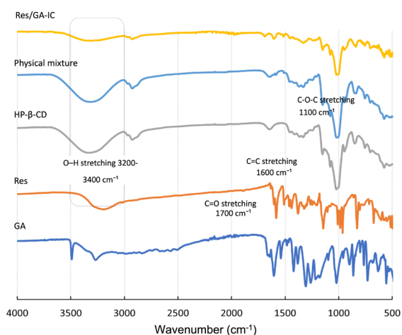
Figure 4. FTIR spectra of Res, GA, HP- \beta -CD, Res and GA physical mixture, and the Res/GA-IC
