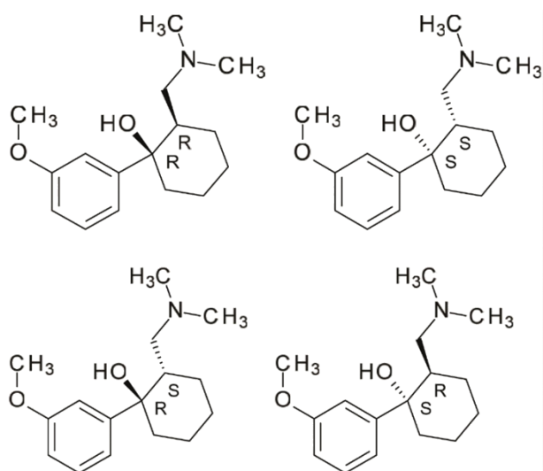
Figure 1. Tramadol enantiomers chemical structures.
