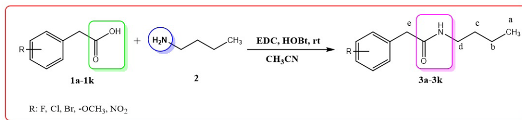
Figure 1. Synthetic pathway of phenylacetamide derivatives 3a-3k .
