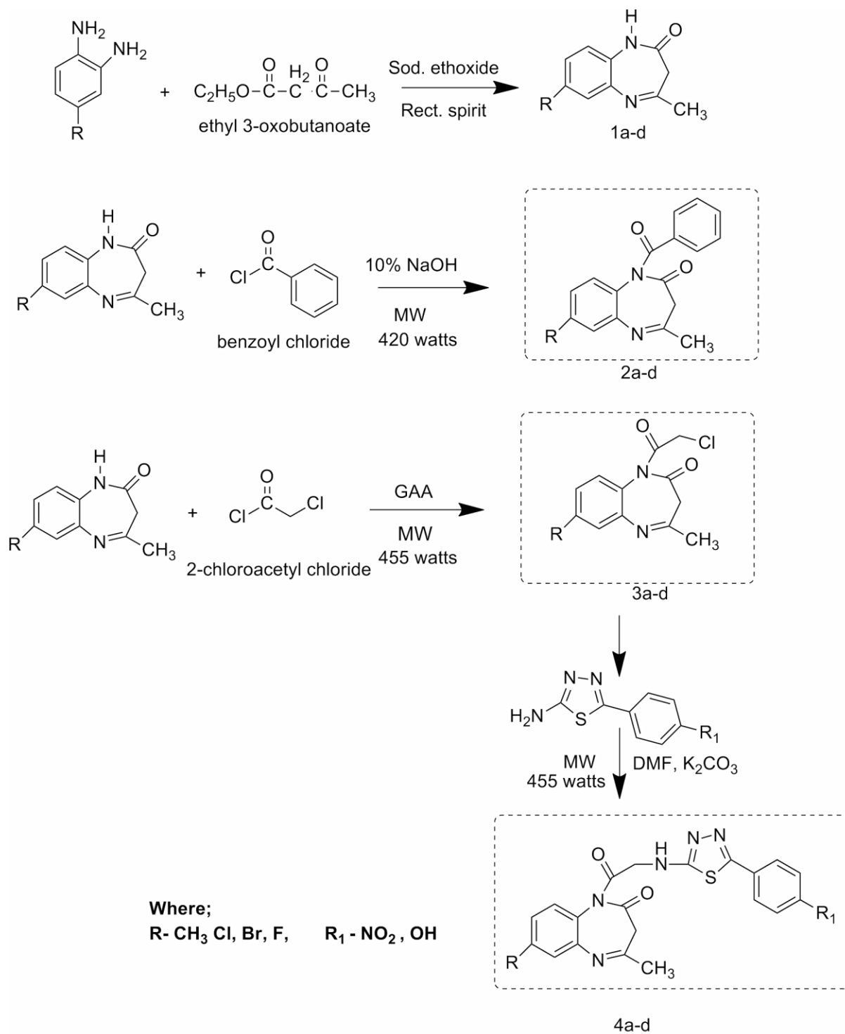
Figure 1. Scheme for synthesis of compound. 1a-d, 3a-d, and 4a-d respectively.
